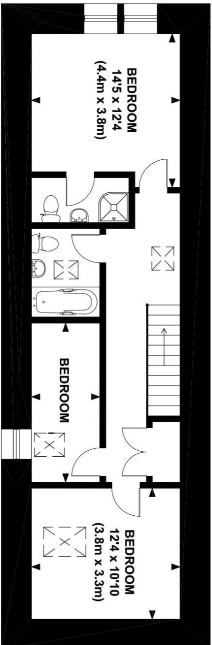
FIRST FLOOR
